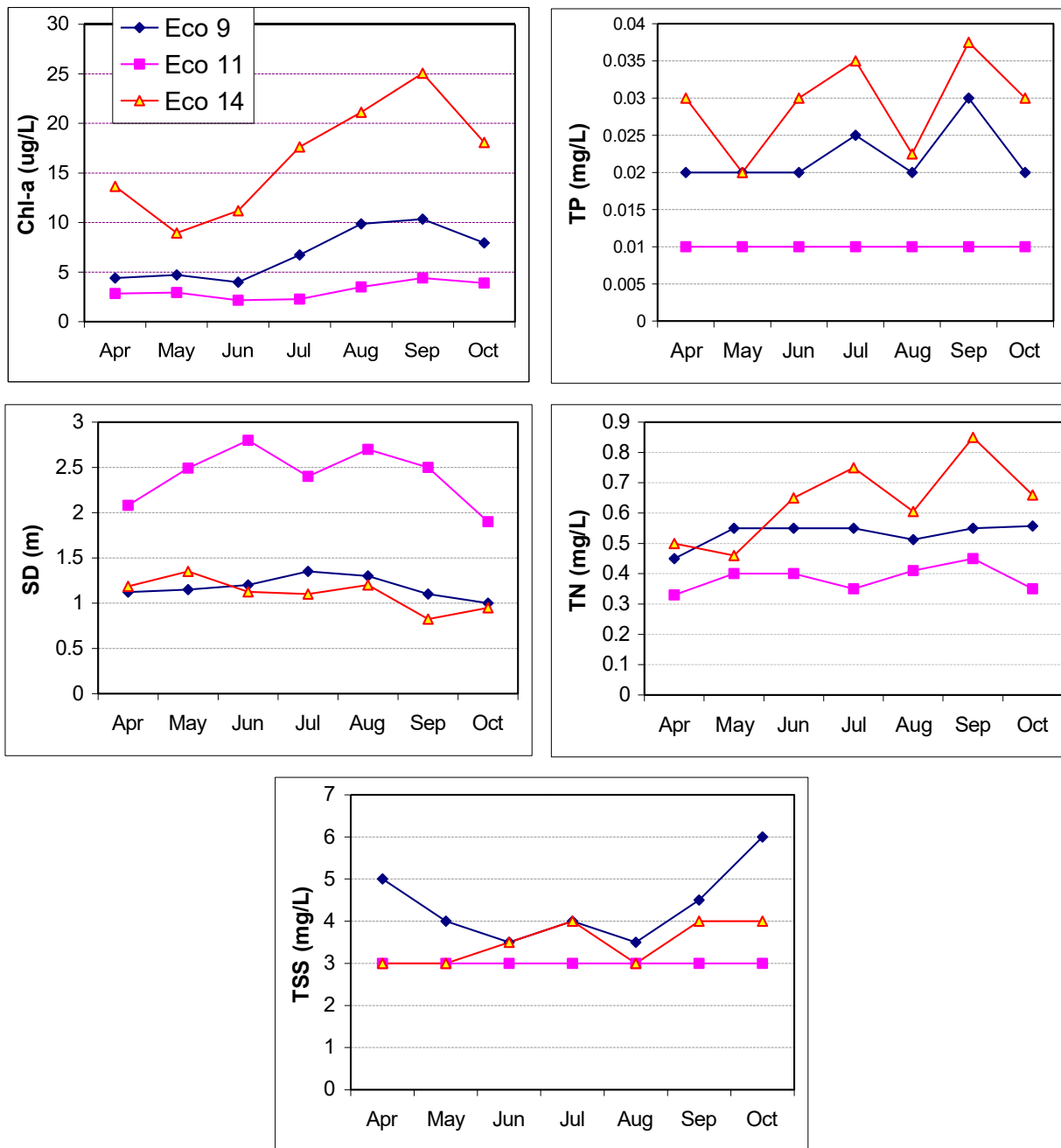
Figure 4. Seasonal variation of nutrient variables and TSS, by ecoregion. The ecoregion 9 plots represent an average of 30 lakes (range = 23 to 36); ecoregion 11 by an average of 16 lakes (range = 15 – 17); and ecoregion 14 by an average of 7 lakes (range = 5 – 8). 3 mg/L TSS and 0.01 mg/L TP represent commonly applied analytical detection limits.
