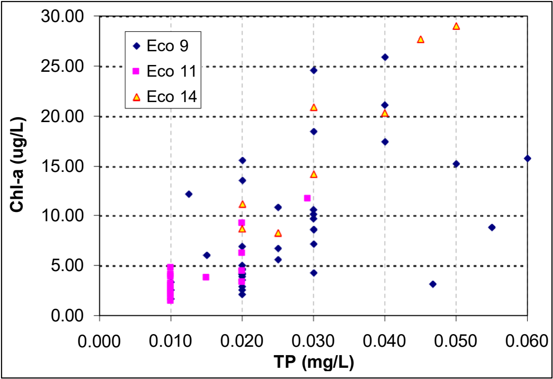
Figure 9. Lake-median (April – October) Chl-a vs. TP concentrations, by ecoregion, for the Virginia impoundments used in this study. Three lakes with Chl-a medians > 50 \mu\text{g/L} (outliers) are not represented.
