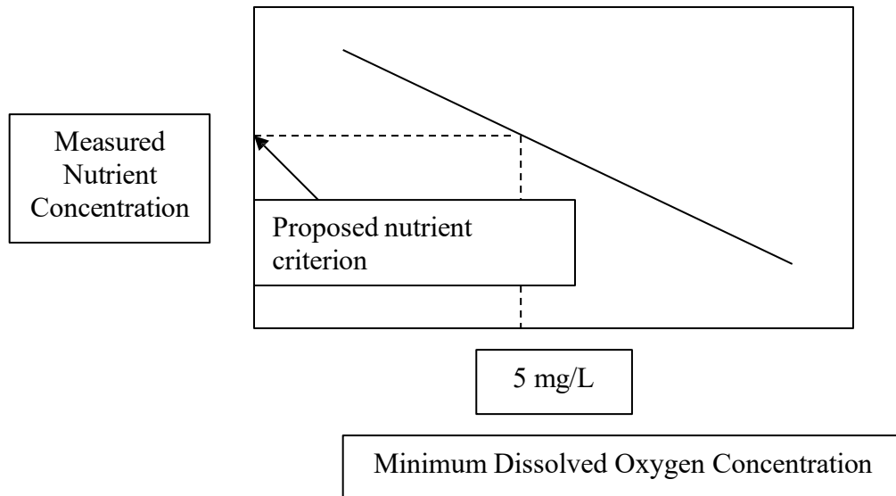
Figure 1. Expected relation between measured nutrients and minimum dissolved oxygen in Region III streams (generalized).
