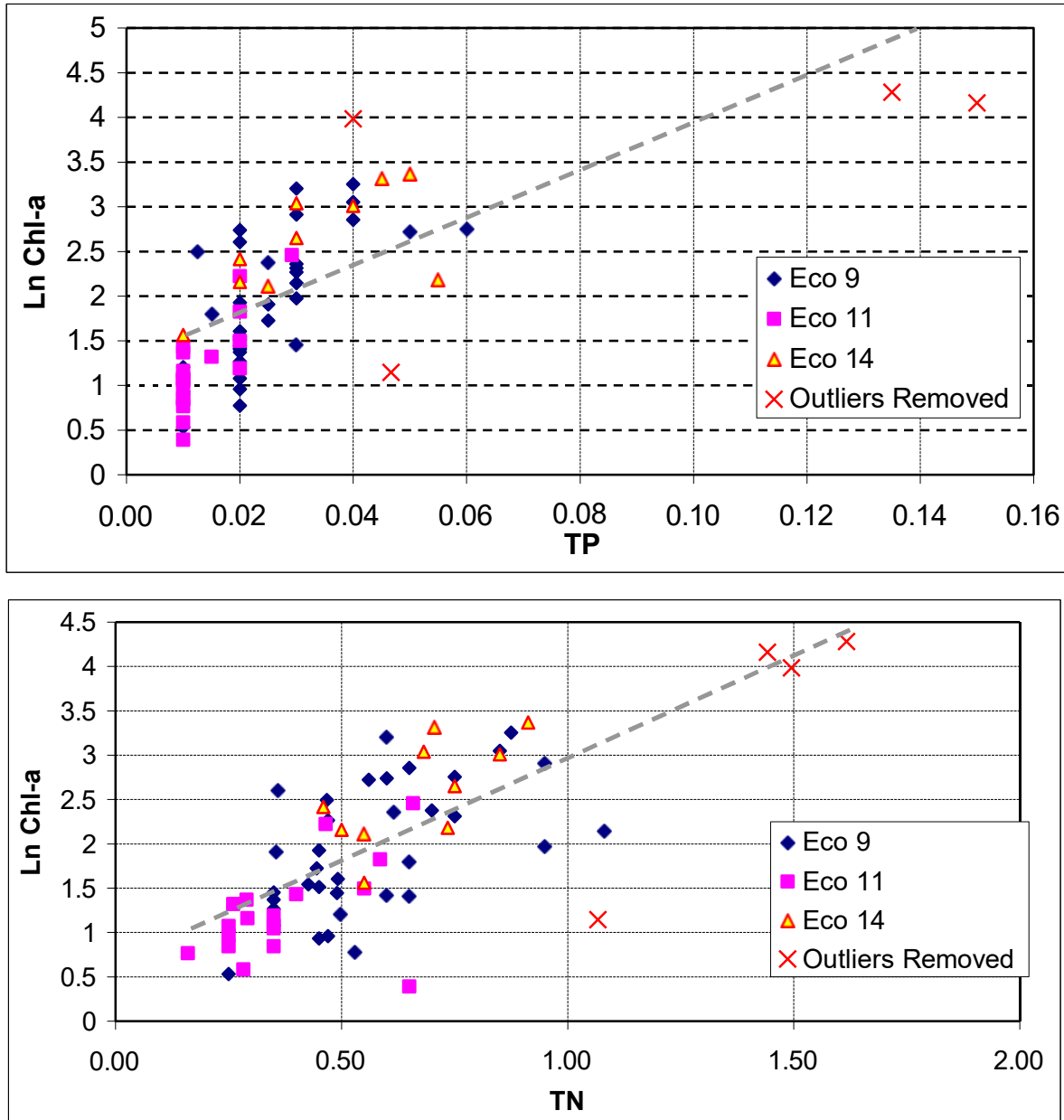
Figure 6. Ln Chl-a as univariate functions of TP and TN. Ecoregions are represented in the plots but were not considered in the regression analyses represented above.
