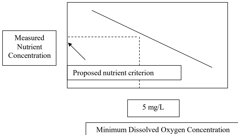
Figure 1. Expected relation between measured nutrients and minimum dissolved oxygen in Region III streams (generalized).
