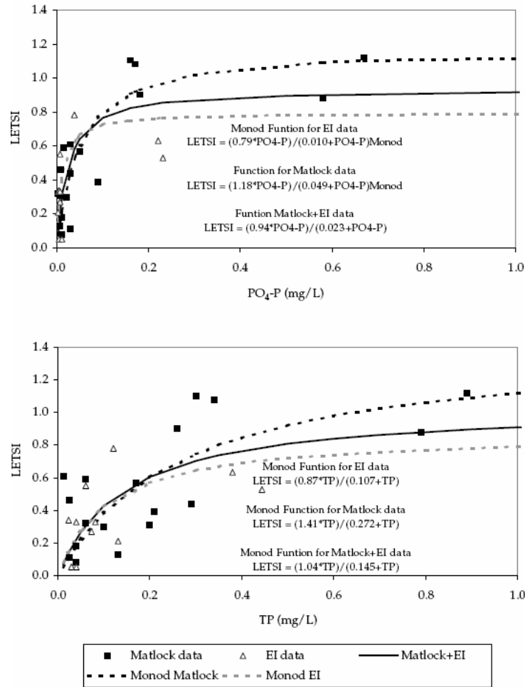
Figure 8. Monod curve fit of PO 4 -P concentrations to LETSI values for P-limited and not limited results. EI = current study [McFarland et al. 2004] and Matlock = Matlock and Rodriguez (1999). X-axis truncated at 1.0 mg/L. 12
