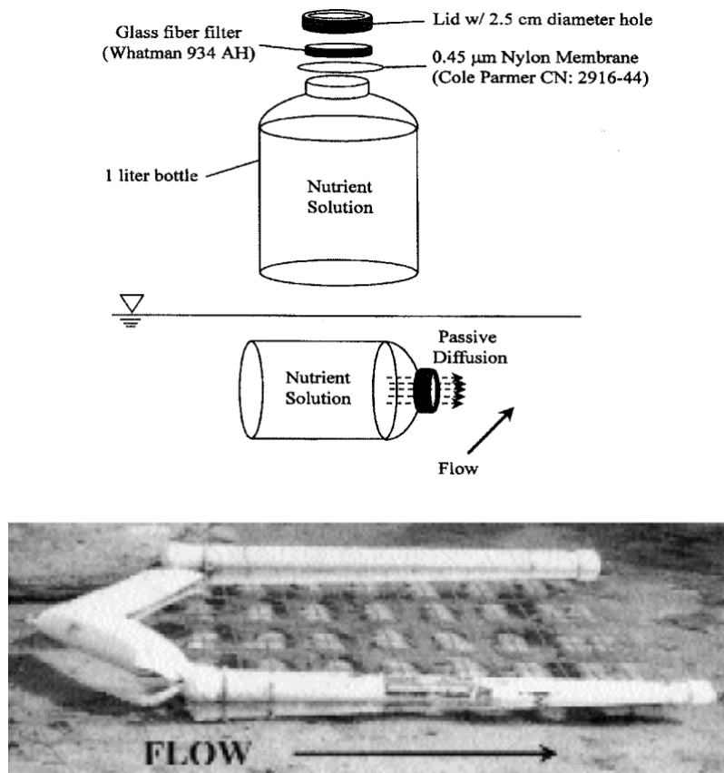
Figure 7. Diagrams of Matlock Periphytometer and photo showing Matlock Periphytometer treatment arrays. 11
