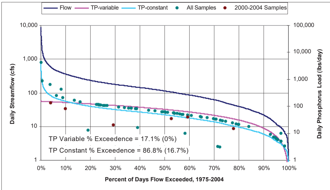
Figure 29. TP Load-Duration Curve for THO006.50.
