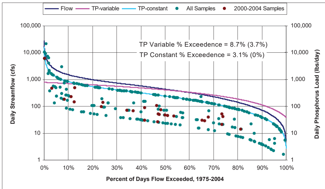
Figure 27. TP Load-Duration Curve for RPP147.10.
