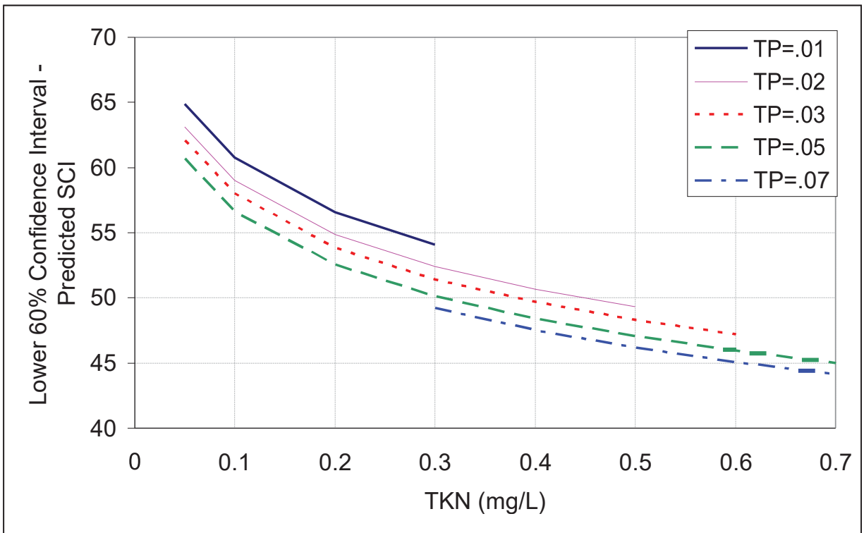
Figure 7. Lower boundaries of the 80% (above) and 60% (below) Stream Condition Index (SCI)-prediction intervals for various (TKN, TP) combinations contained within the data set, as per the bivariate (TKN, TP) SCI prediction model.
