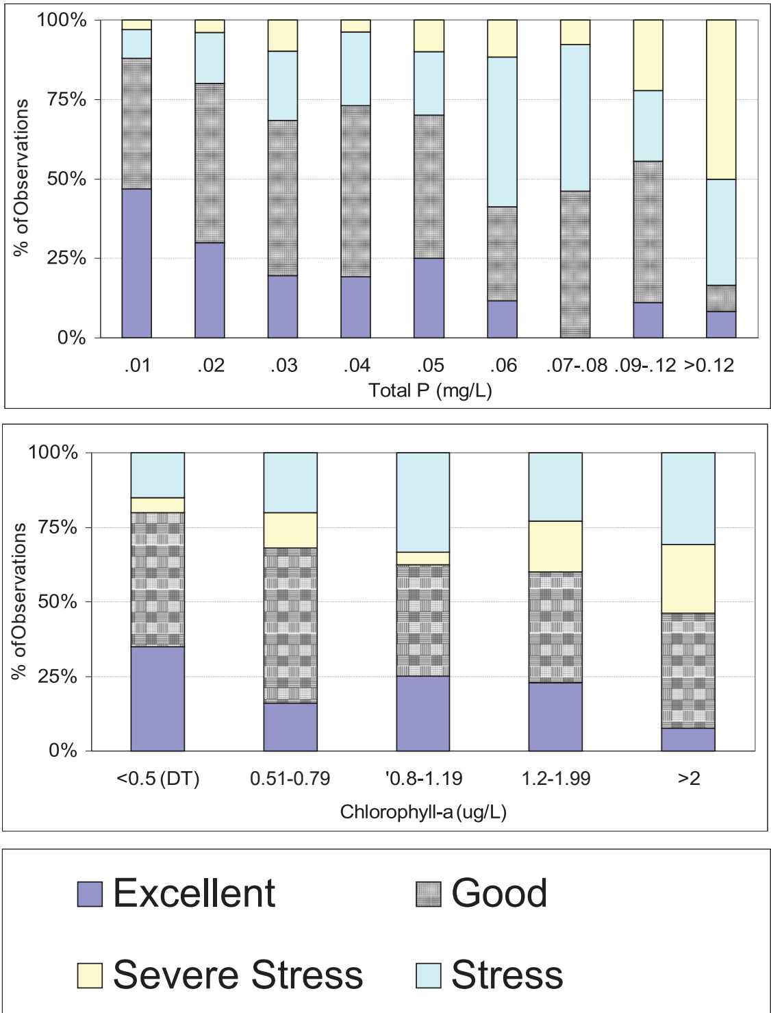
Figure 5. Histograms representing percentages of benthic macroinvertebrate observations within various aquatic life use tiers occurring within different nutrient categories. Stressed and severely stressed communities are defined as impaired. Histograms for nitrogen water-quality variables are displayed on the following page.
