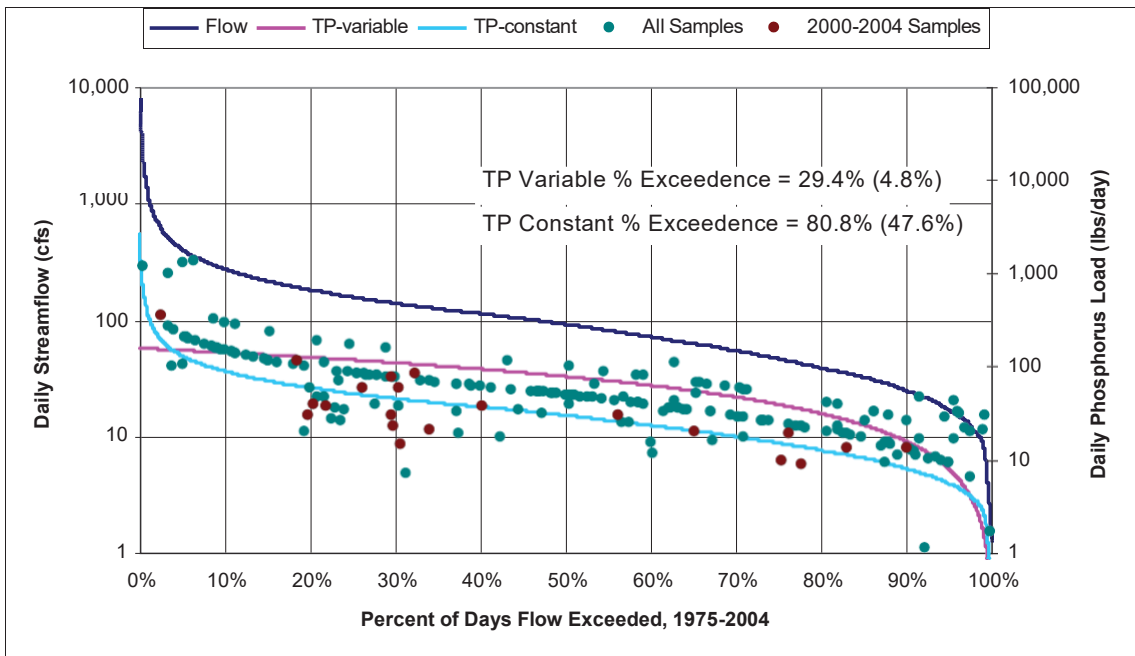
Figure 19. TP Load-Duration Curve for LDR000.70.
