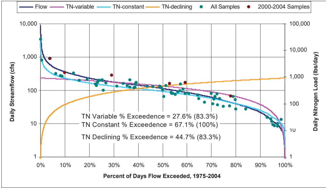
Figure 28. TN Load-Duration Curve for THO006.50.
