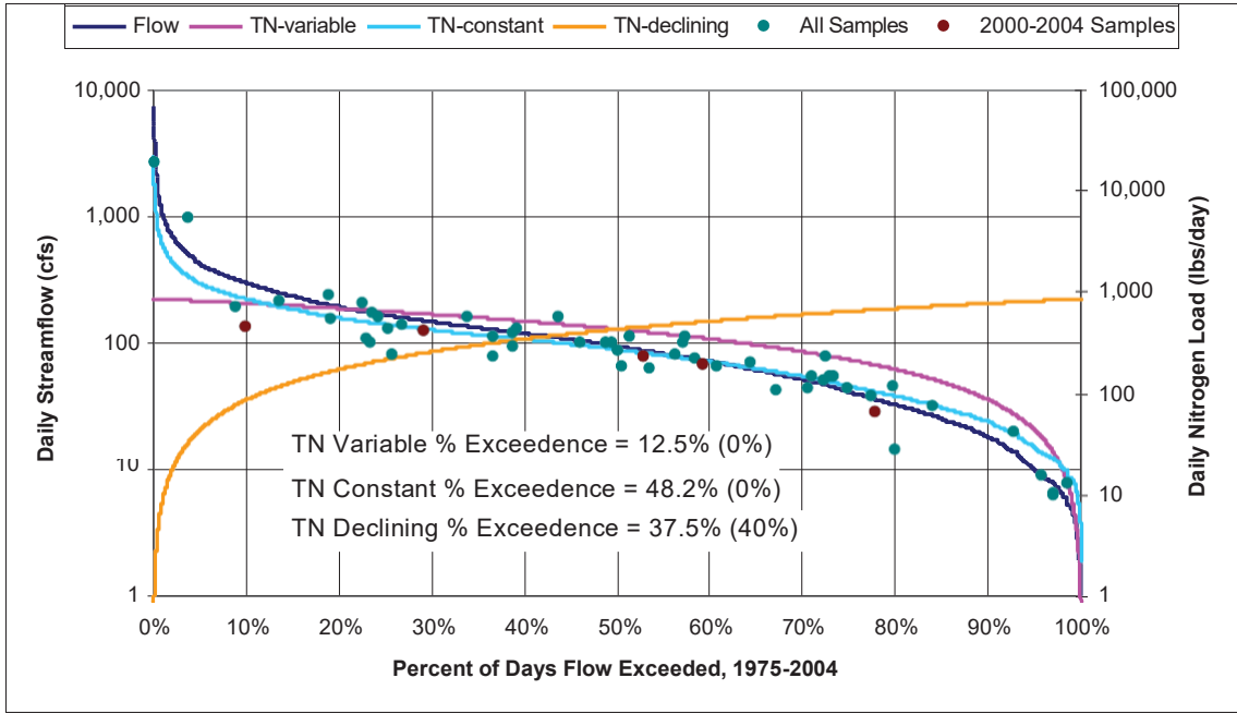
Figure 16. TN Load-Duration Curve for HAZ018.29.
