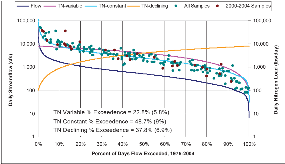
Figure 20. TN Load-Duration Curve for RAP006.53.
