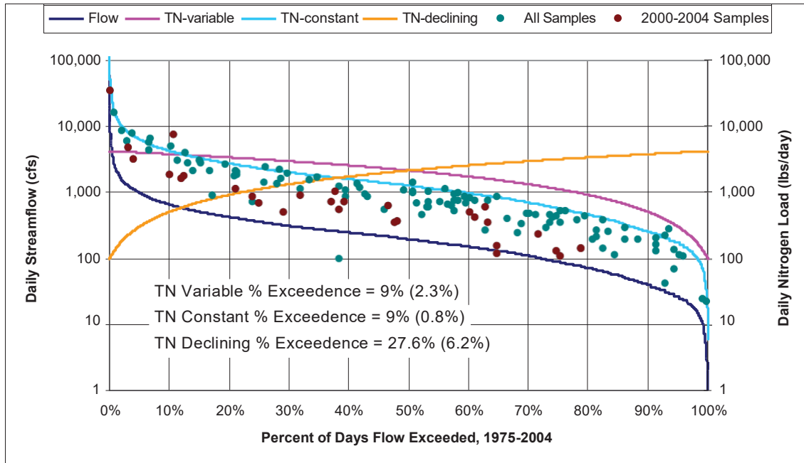
Figure 22. TN Load-Duration Curve for RAP045.08.
