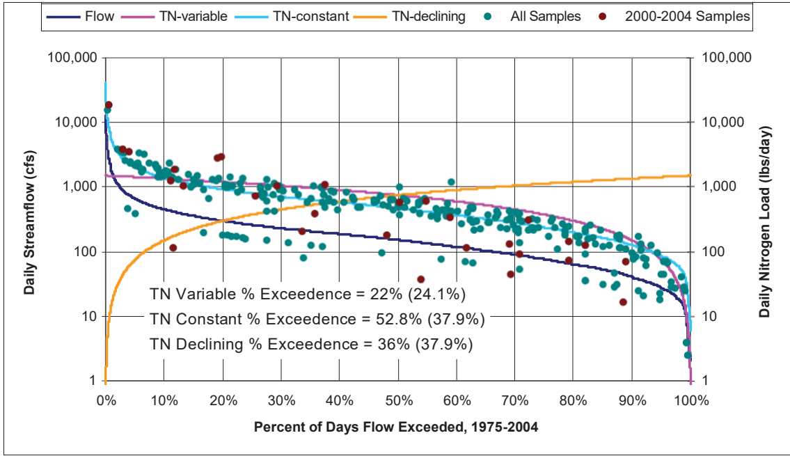
Figure 24. TN Load-Duration Curve for ROB001.90.
