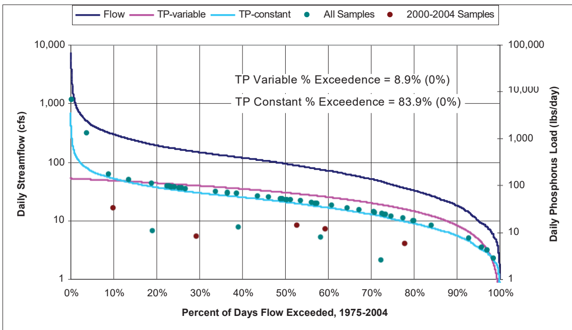
Figure 17. TP Load-Duration Curve for HAZ018.29.
