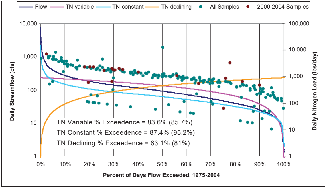
Figure 18. TN Load-Duration Curve for LDR000.70.
