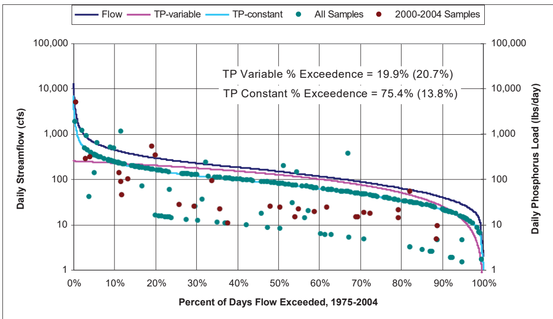
Figure 25. TP Load-Duration Curve for ROB001.90.
