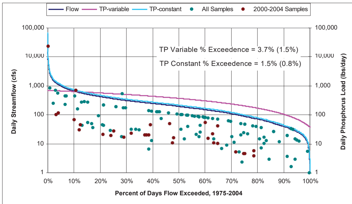
Figure 23. TP Load-Duration Curve for RAP045.08.
