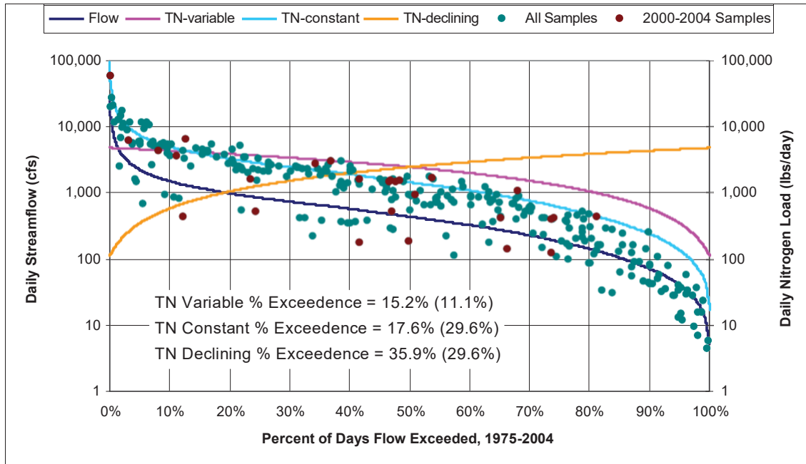
Figure 26. TN Load-Duration Curve for RPP147.10.
