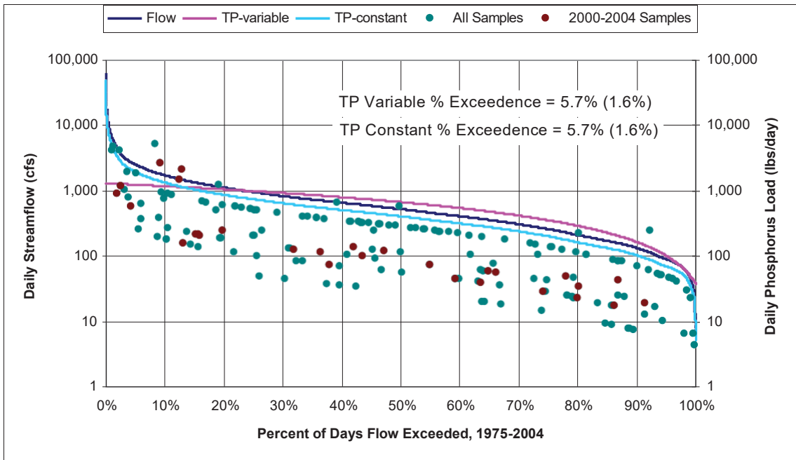
Figure 21. TP Load-Duration Curve for RAP006.53.
